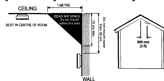
Figure 3i- Positioning the smoke / heat detector Figure 3ii
